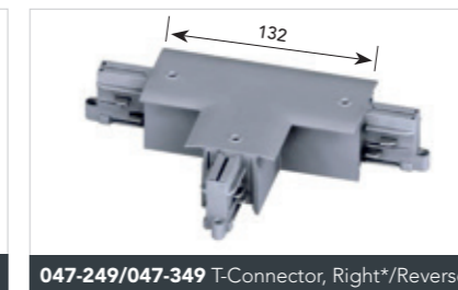
047-249/047-349 T-Connector, Right*/Reverse*
